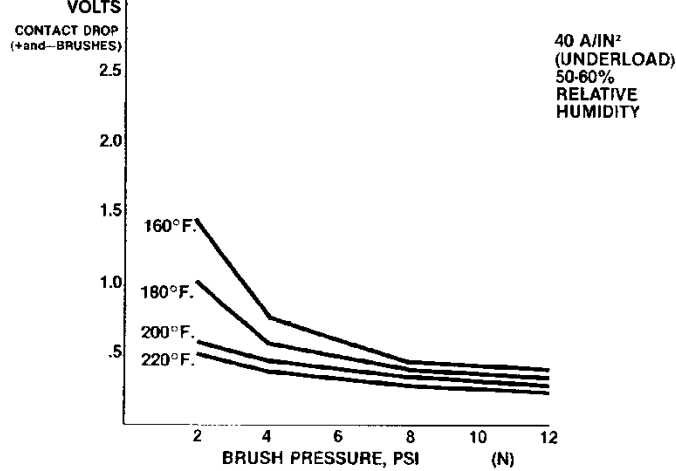
GRAPH III EFFECT OF PRESSURE ON VOLTAGE DROP
