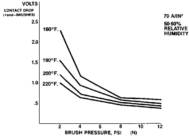
GRAPH II EFFECT OF PRESSURE ON VOLTAGE DROP
