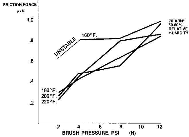
GRAPH I EFFECT OF PRESSURE ON FRICTION
