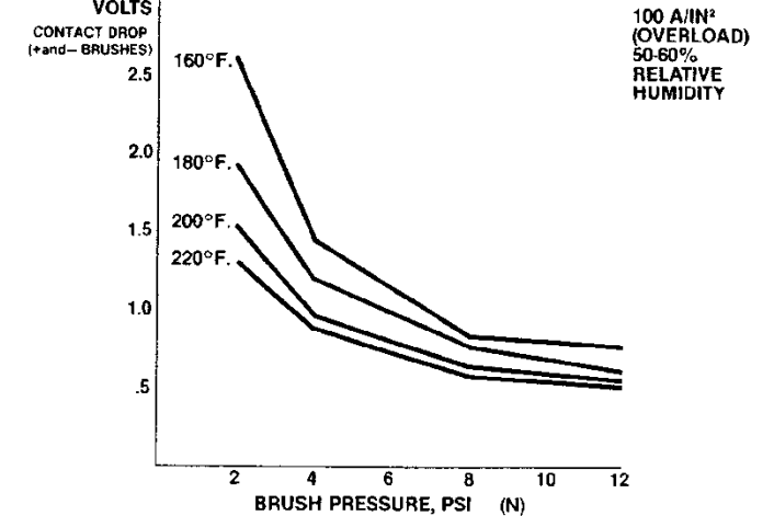
GRAPH IV EFFECT OF PRESSURE ON VOLTAGE DROP
