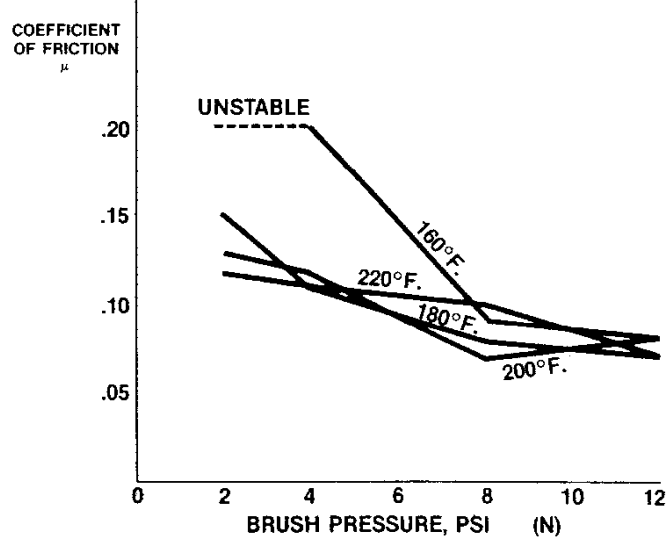
GRAPH IA EFFECT OF PRESSURE ON COEFFICIENT OF FRICTION
